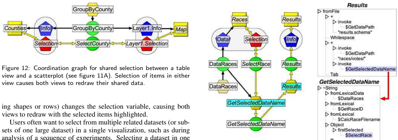
Figure 13: Coordinated query graph for selection-dependent loading of data (see figure 11B). An index on the races dataset maps the record identifier of the first selected race into a filename. The “Results” view displays an info (an expression that calculates a dataset) that reads data from the corresponding file of voting results.
